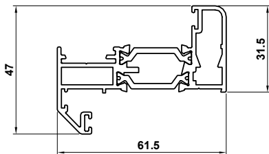
ETC321 Externally Glazed Sash System 2
