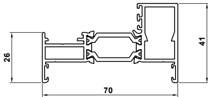
ZSB169 Outer Frame
