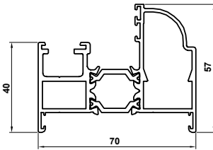
ETD015 Outer Frame
