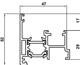
ETD048 Dummy Mullion
