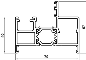
ETD017 Outer Frame
