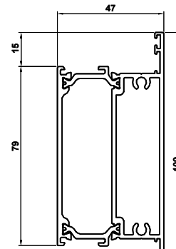
ETD033 Midrail use with ETD025N
